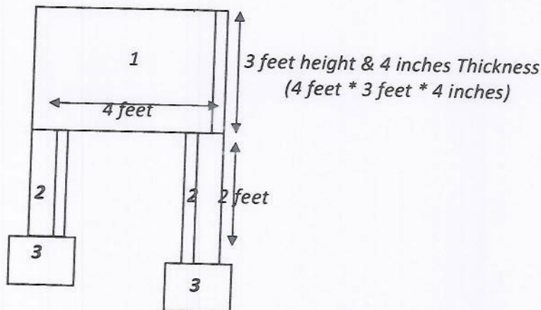
Pre cast slab (2 nos on each leg) 1' X 1' X 0'.4"
